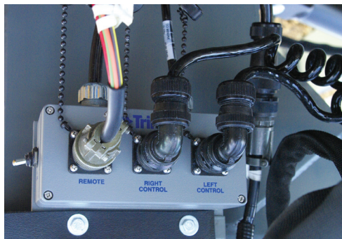
502415 Laser Install Kit (Junction Box Assembly)
